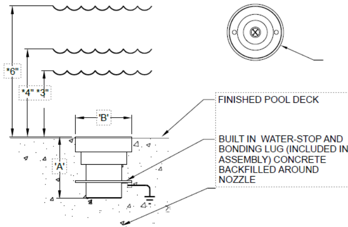
N-FN-100 ELEVATION
